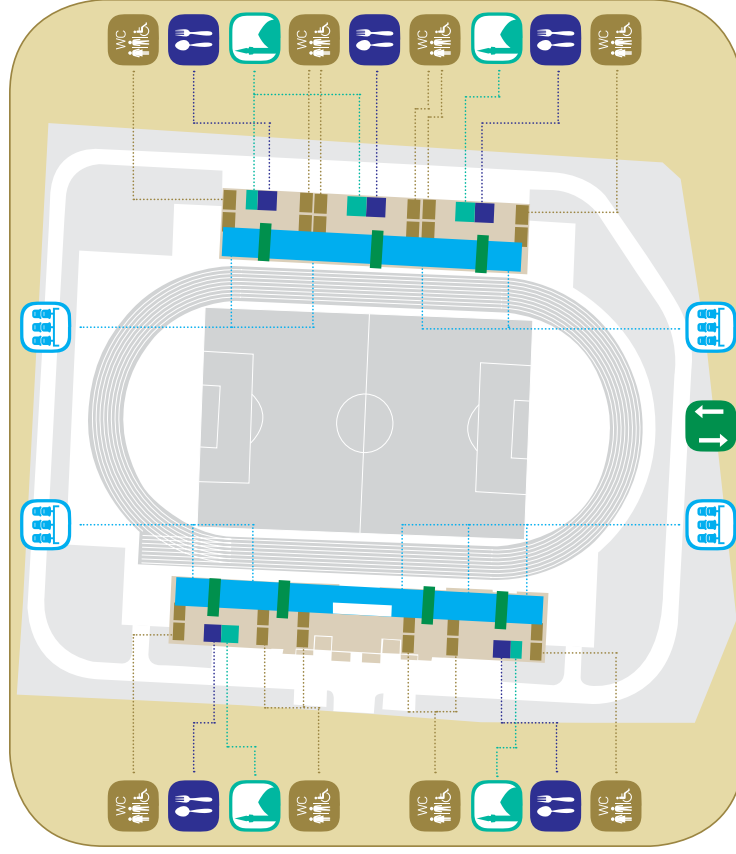
FIELD LAYOUT
